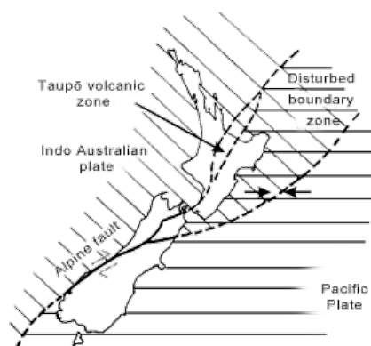
Earth's tectonic plates and New Zealand
